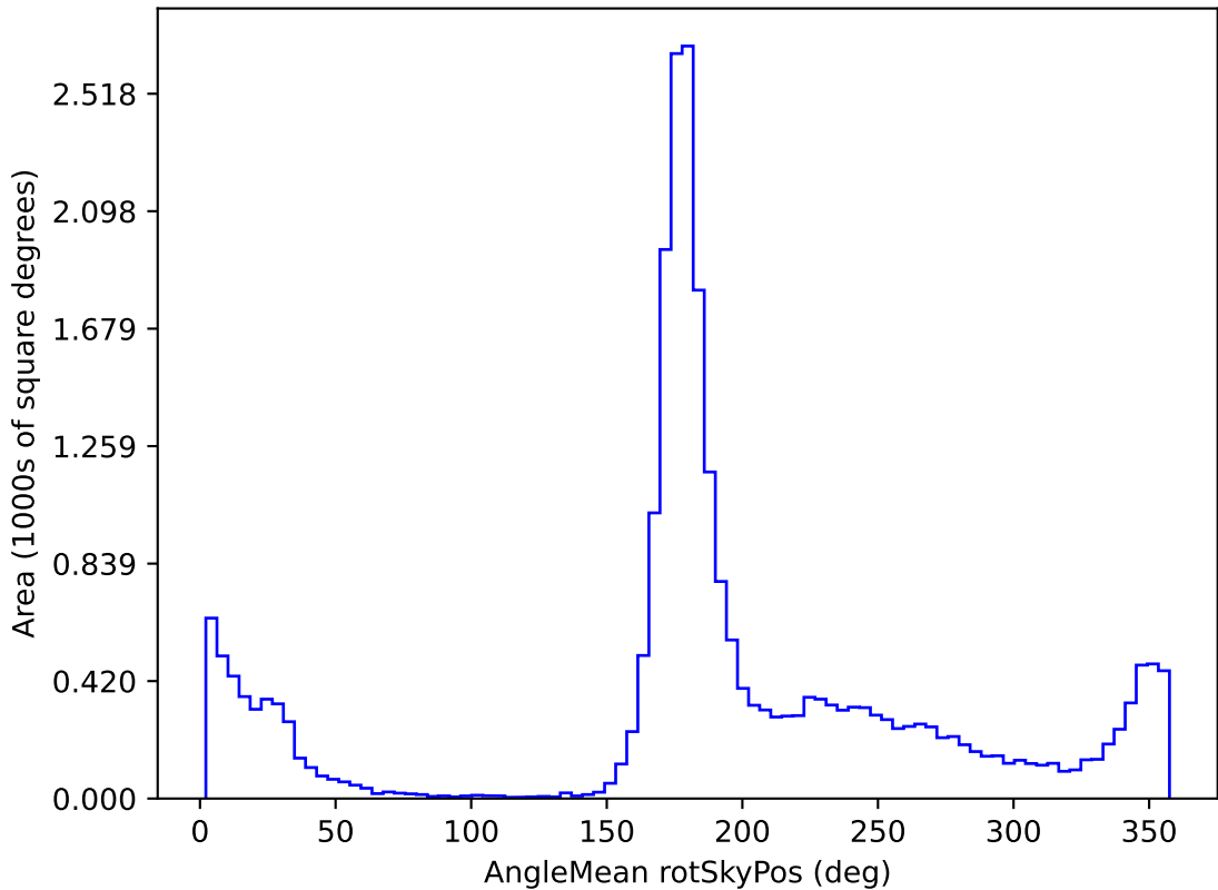
roll_pause_mjdp365_v3.4_10yrs All sky r band: AngleMean rotSkyPos
