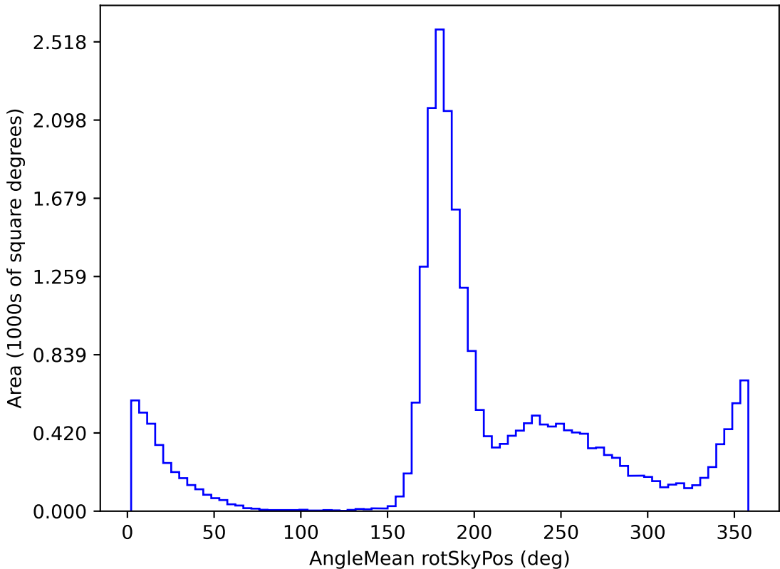
roll_pause_mjdp365_v3.4_10yrs All sky i band: AngleMean rotSkyPos
