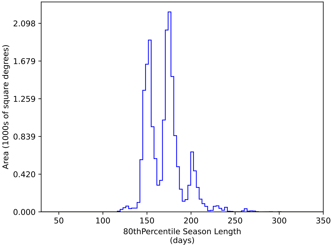
roll_pause_mjdp365_v3.4_10yrs WFD y band: 80thPercentile Season Length
