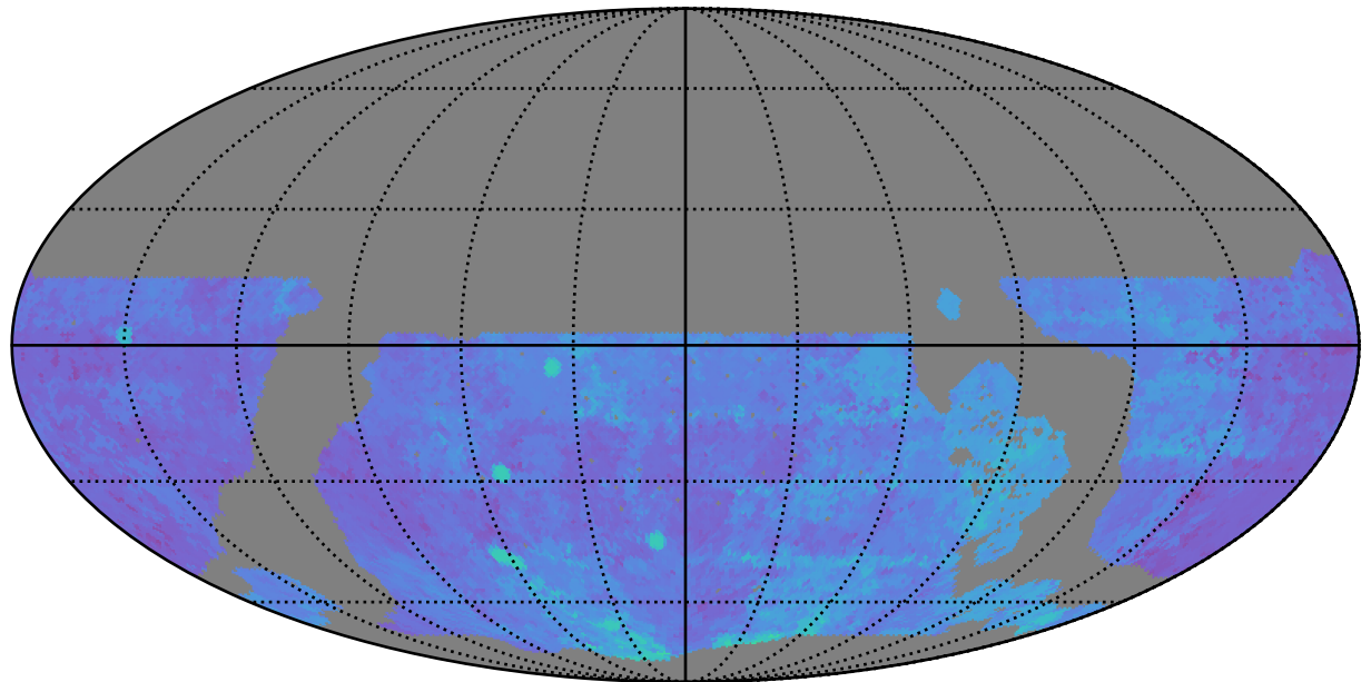
roll_pause_mjdp365_v3.4_10yrs WFD g band: 80thPercentile Season Length
