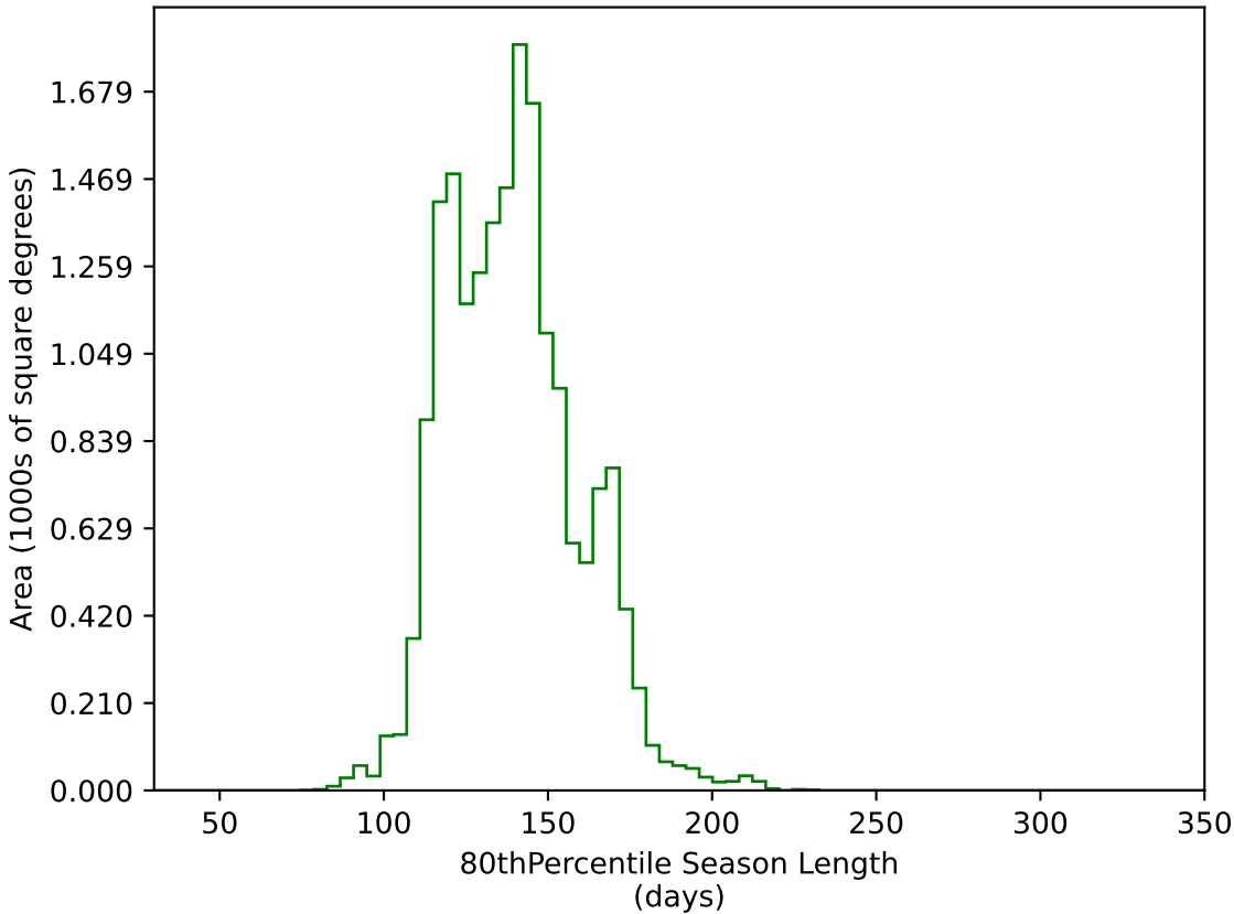
roll_pause_mjdp365_v3.4_10yrs WFD g band: 80thPercentile Season Length
