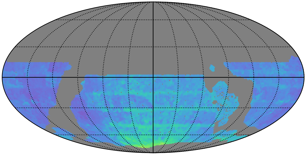
roll_pause_mjdp365_v3.4_10yrs WFD all bands: 80thPercentile Season Length
