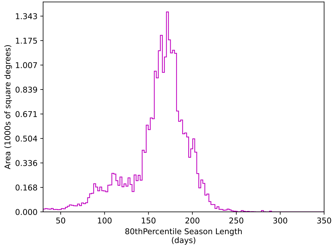
roll_pause_mjdp365_v3.4_10yrs All sky z band: 80thPercentile Season Length
