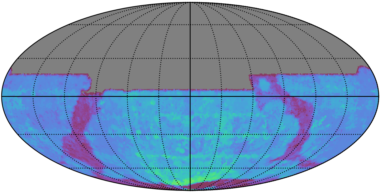
roll_pause_mjdp365_v3.4_10yrs All sky y band: 80thPercentile Season Length
