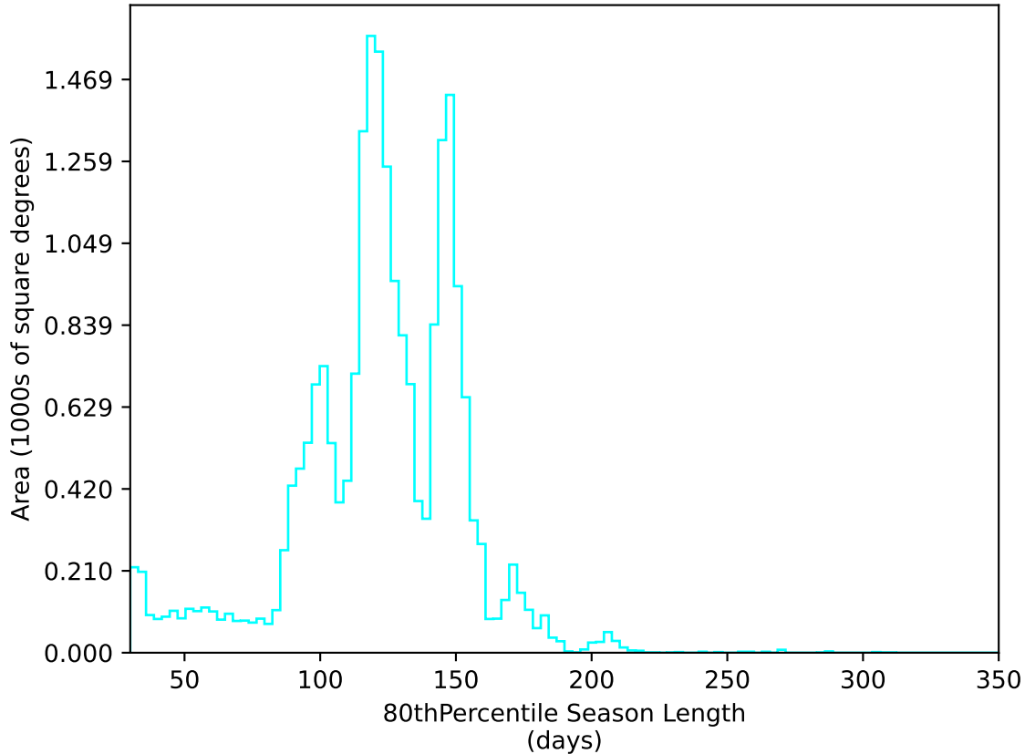
roll_pause_mjdp365_v3.4_10yrs All sky u band: 80thPercentile Season Length
