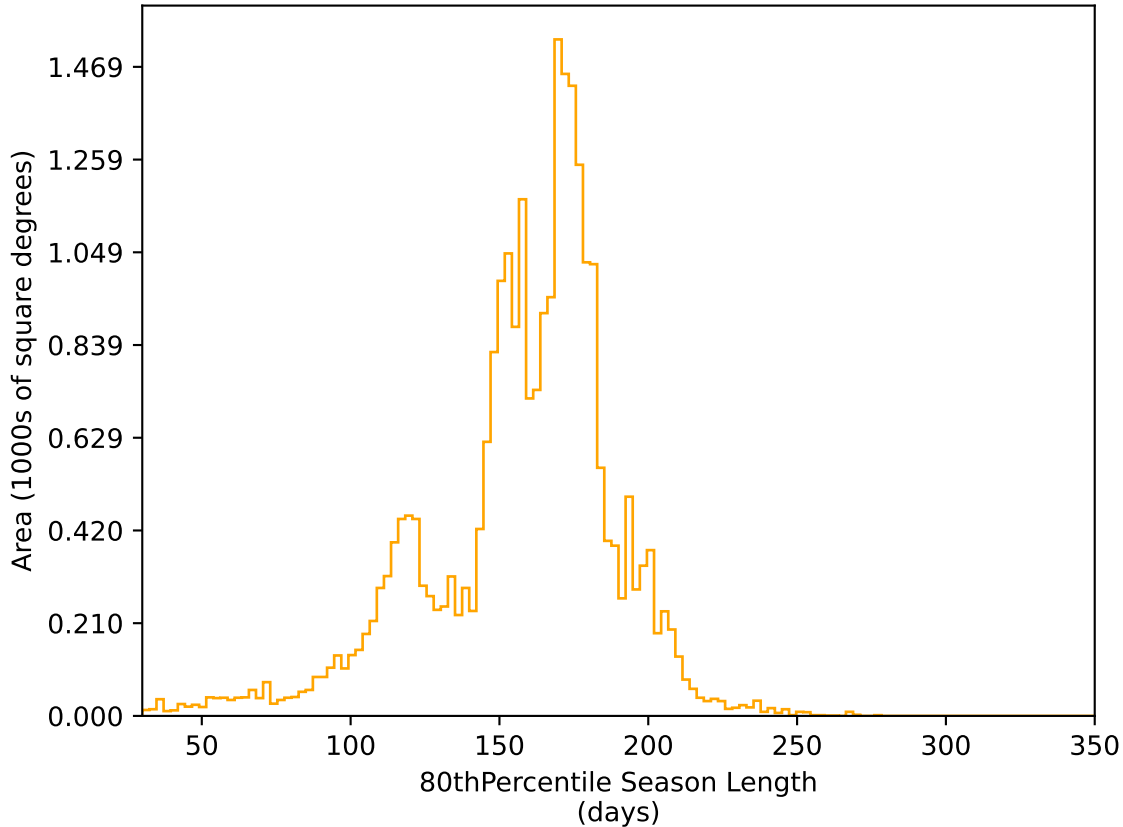
roll_pause_mjdp365_v3.4_10yrs All sky r band: 80thPercentile Season Length
