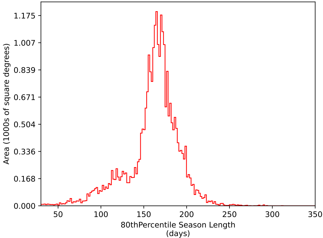
roll_pause_mjdp365_v3.4_10yrs All sky i band: 80thPercentile Season Length
