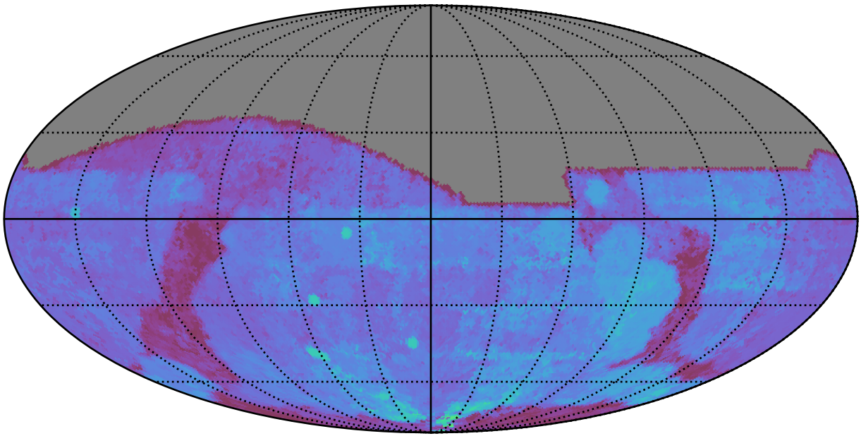
roll_pause_mjdp365_v3.4_10yrs All sky g band: 80thPercentile Season Length
