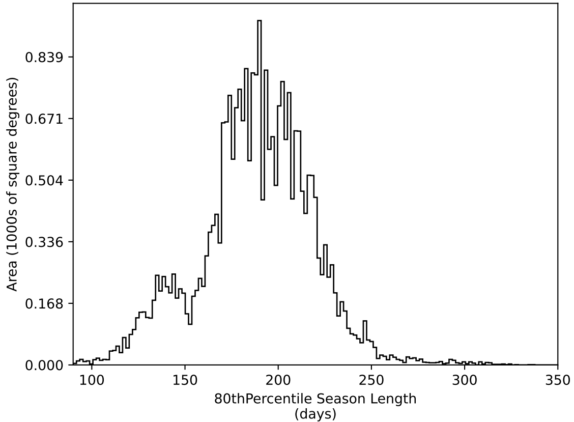
roll_pause_mjdp365_v3.4_10yrs All sky all bands: 80thPercentile Season Length
