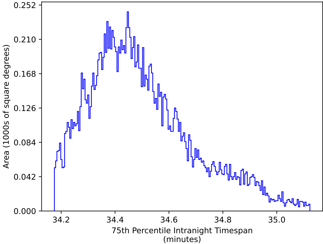
roll_pause_mjdp365_v3.4_10yrs WFD zy bands: 75th Percentile Intranight Timespan
