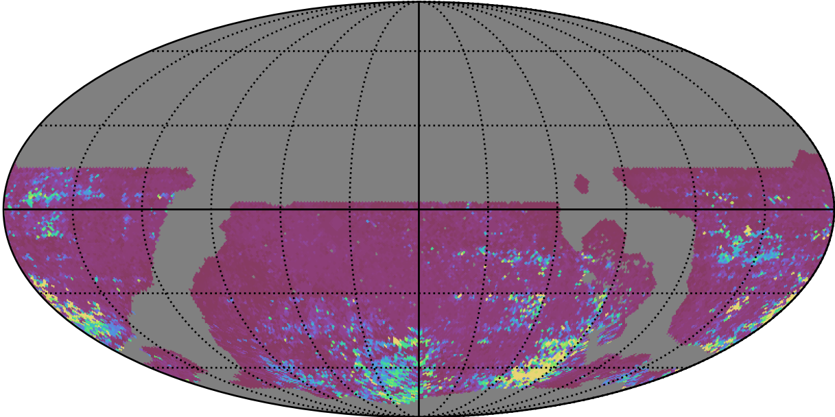
roll_pause_mjdp365_v3.4_10yrs WFD z band: 75th Percentile Intranight Timespan
