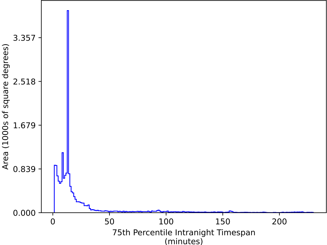
roll_pause_mjdp365_v3.4_10yrs WFD z band: 75th Percentile Intranight Timespan
