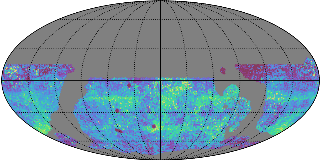
roll_pause_mjdp365_v3.4_10yrs WFD y band: 75th Percentile Intranight Timespan
