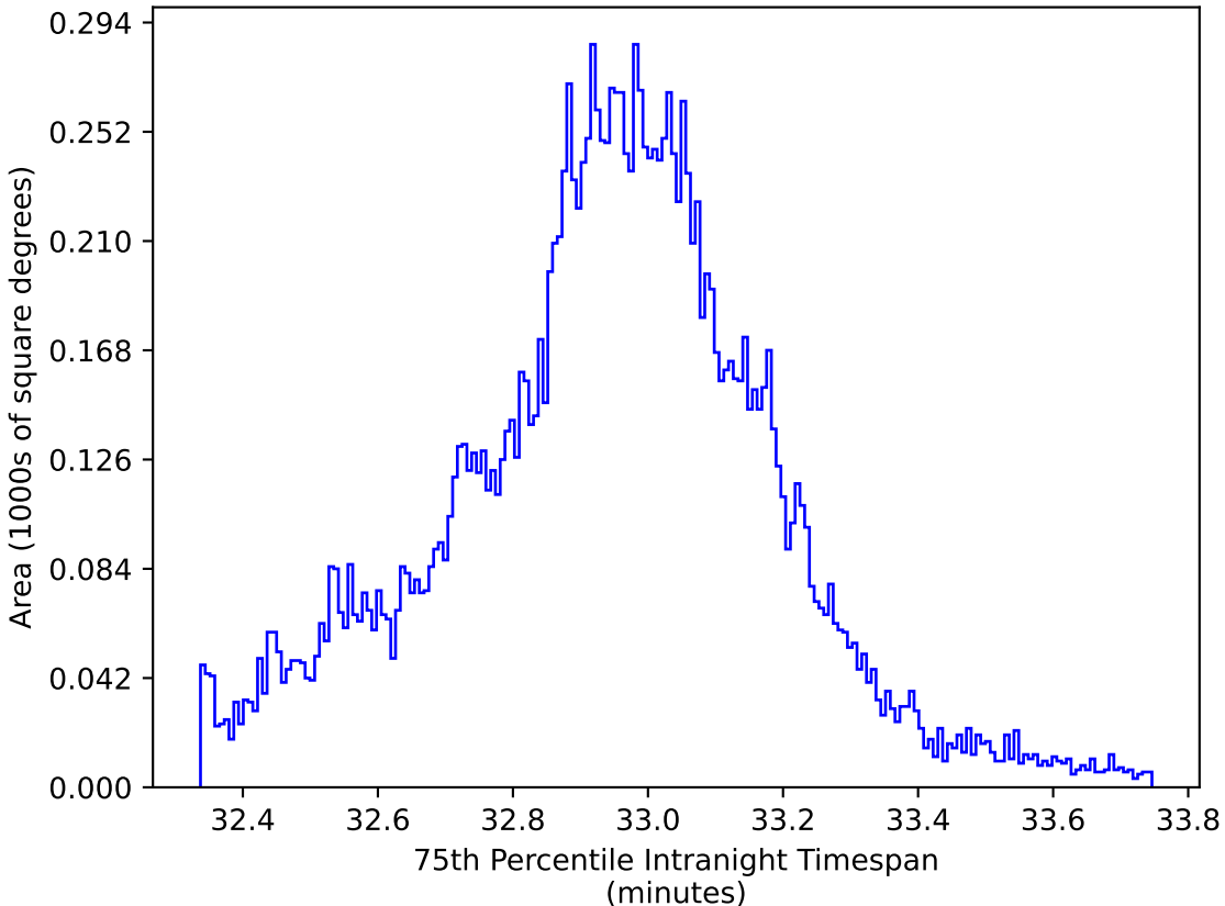
roll_pause_mjdp365_v3.4_10yrs WFD y band: 75th Percentile Intranight Timespan
