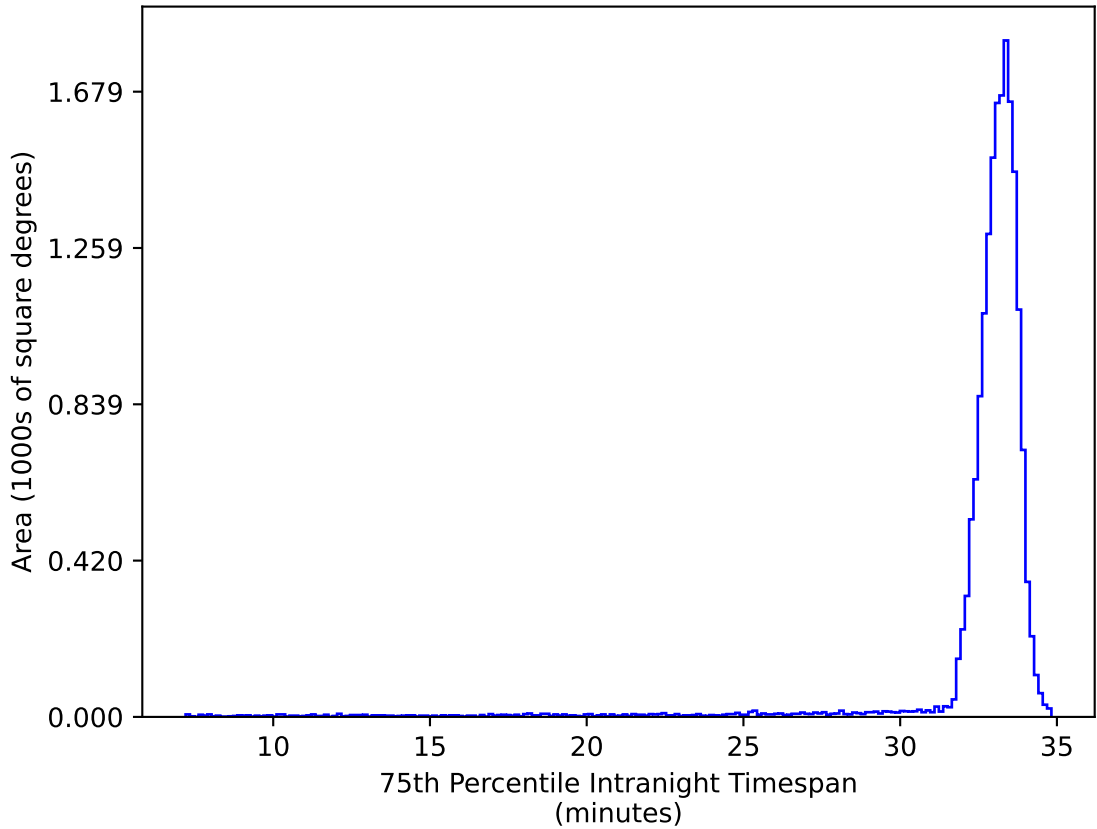
roll_pause_mjdp365_v3.4_10yrs WFD ug bands: 75th Percentile Intranight Timespan
