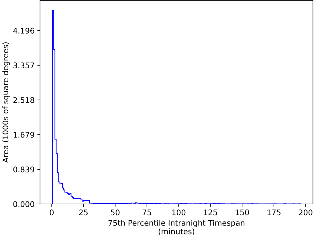
roll_pause_mjdp365_v3.4_10yrs WFD u band: 75th Percentile Intranight Timespan
