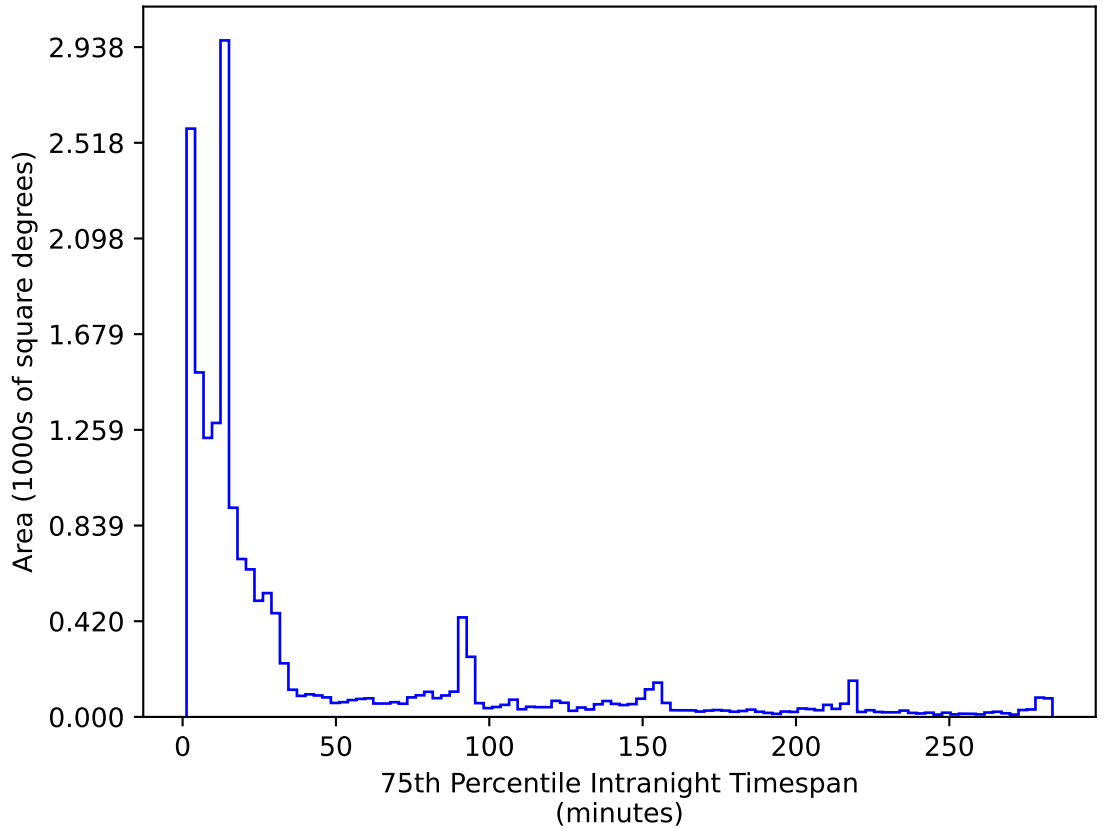
roll_pause_mjdp365_v3.4_10yrs WFD r band: 75th Percentile Intranight Timespan
