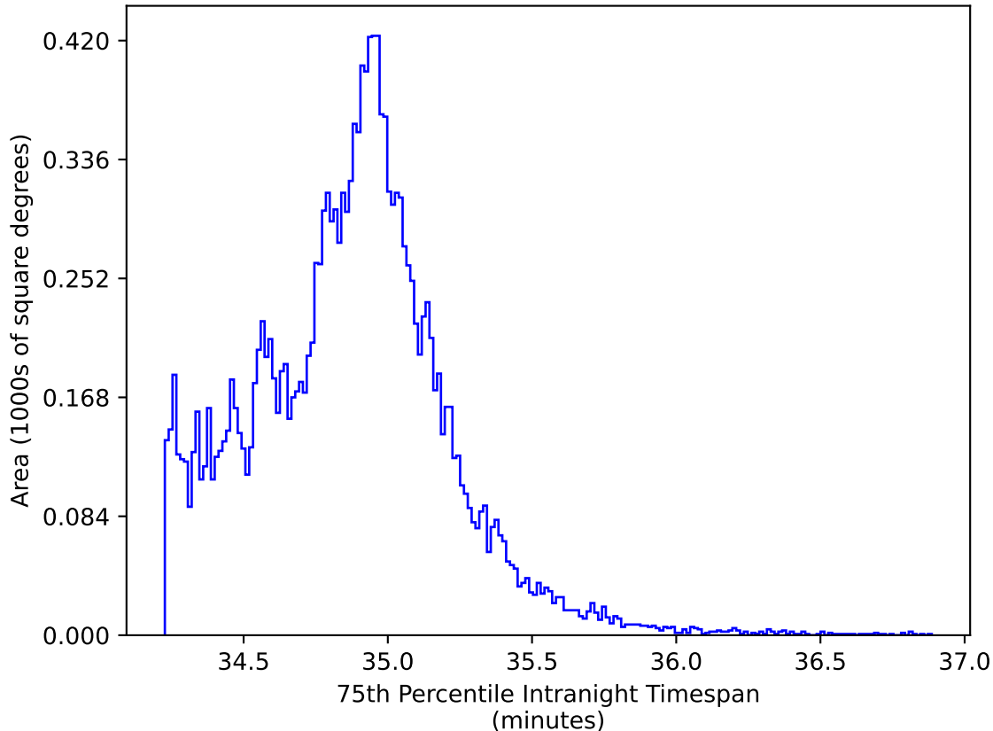
roll_pause_mjdp365_v3.4_10yrs WFD iz bands: 75th Percentile Intranight Timespan
