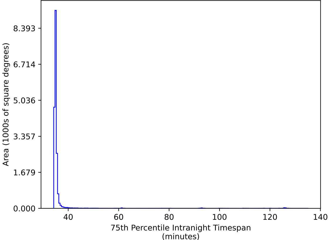
roll_pause_mjdp365_v3.4_10yrs WFD gr bands: 75th Percentile Intranight Timespan
