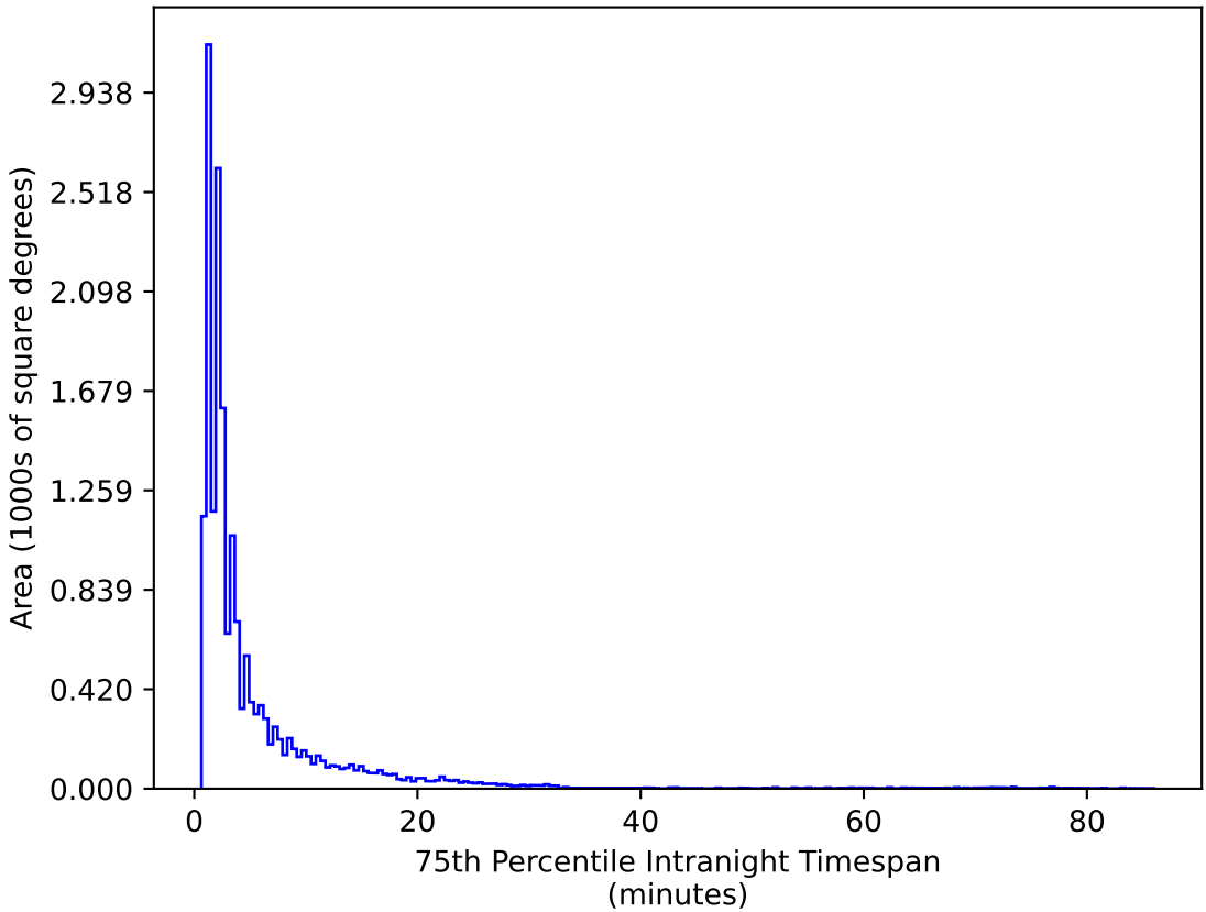
roll_pause_mjdp365_v3.4_10yrs WFD g band: 75th Percentile Intranight Timespan
