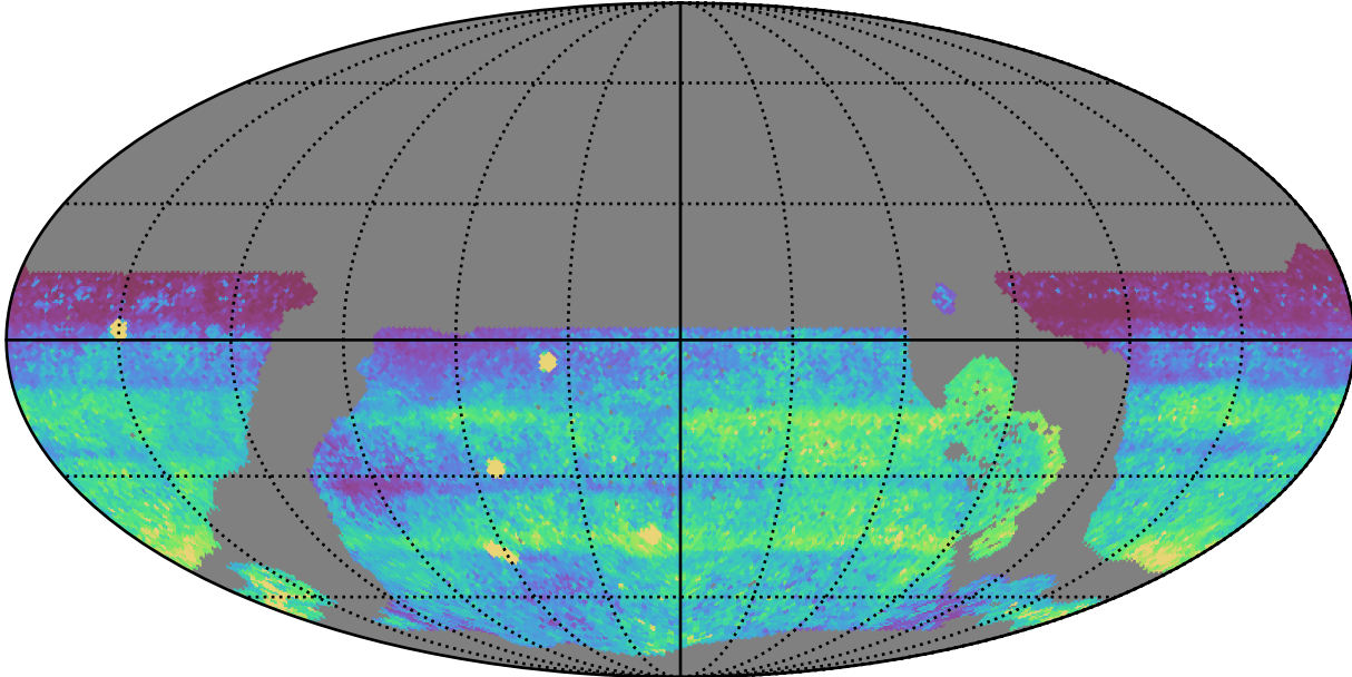
roll_pause_mjdp365_v3.4_10yrs WFD all bands: 75th Percentile Intranight Timespan
