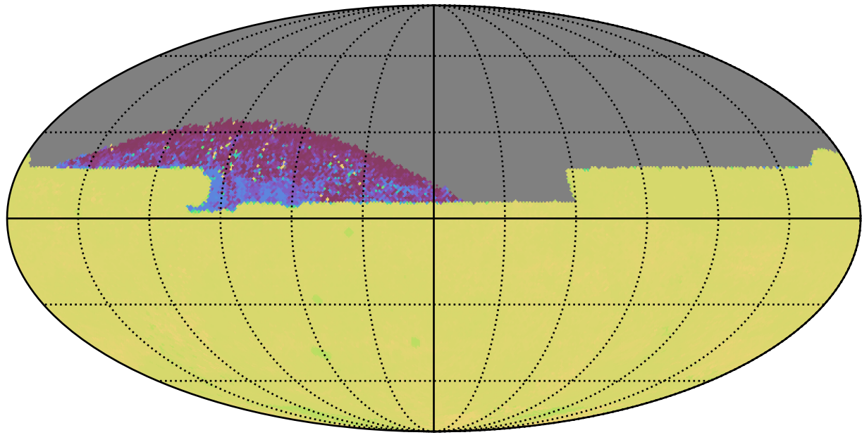
roll_pause_mjdp365_v3.4_10yrs All sky zy bands: 75th Percentile Intranight Timespan
