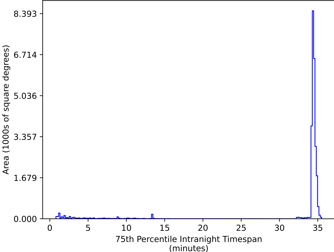
roll_pause_mjdp365_v3.4_10yrs All sky zy bands: 75th Percentile Intranight Timespan
