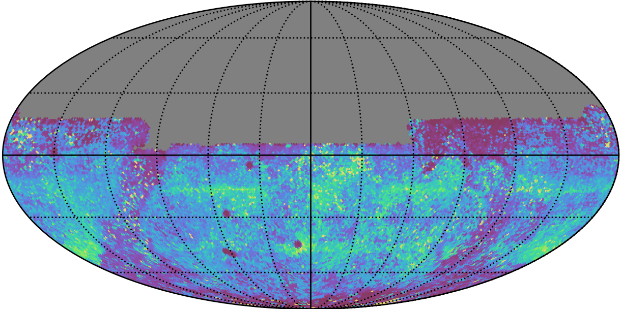
roll_pause_mjdp365_v3.4_10yrs All sky y band: 75th Percentile Intranight Timespan
