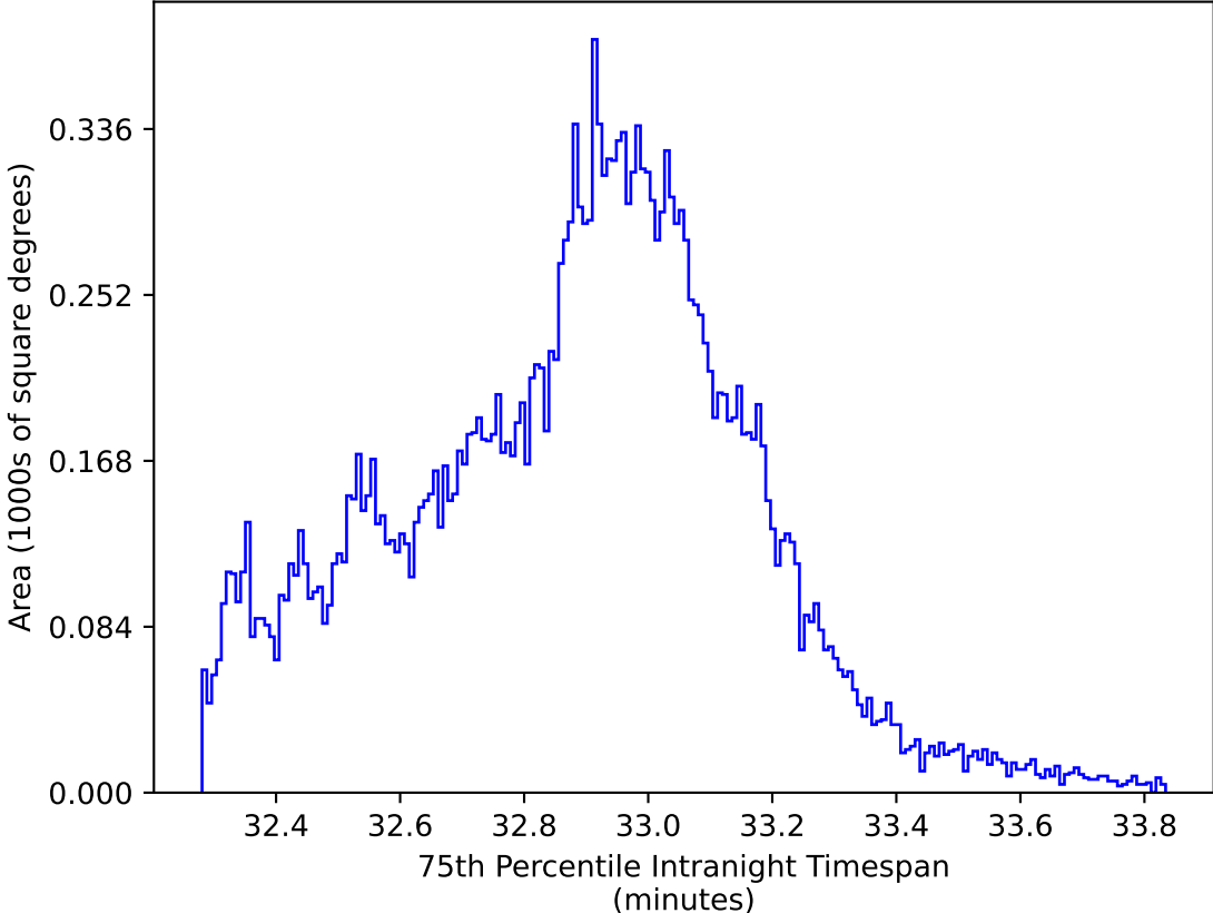
roll_pause_mjdp365_v3.4_10yrs All sky y band: 75th Percentile Intranight Timespan
