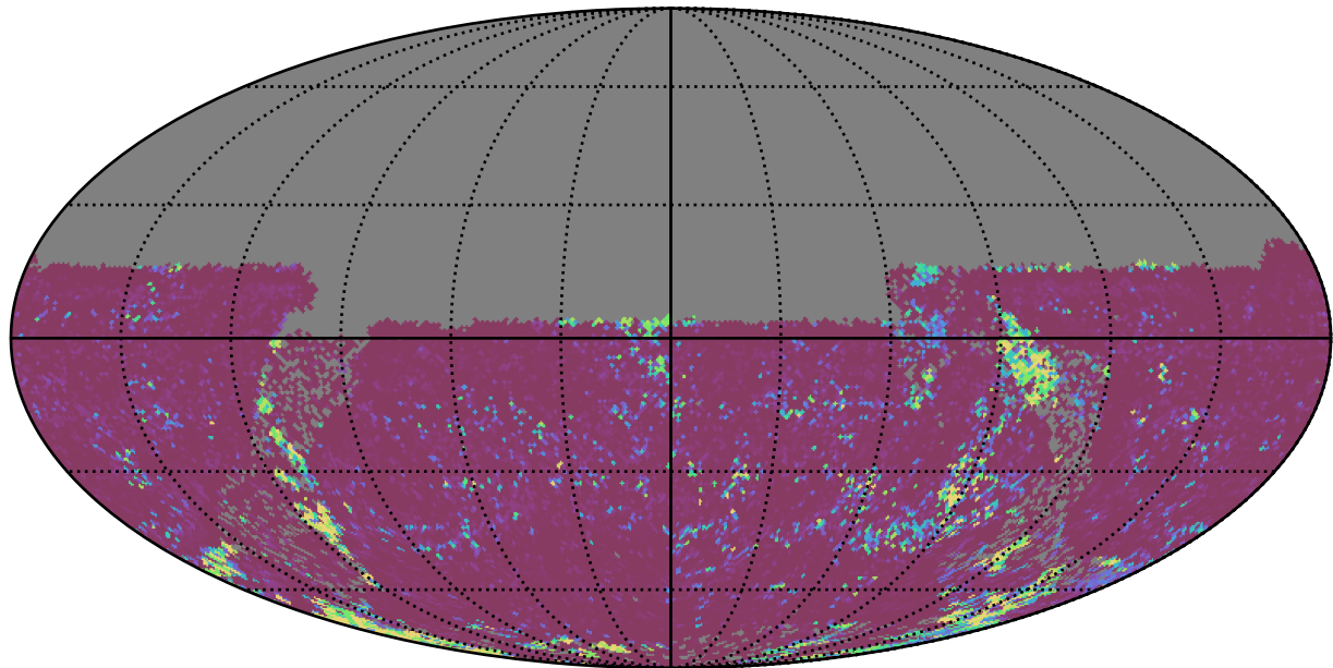
roll_pause_mjdp365_v3.4_10yrs All sky u band: 75th Percentile Intranight Timespan
