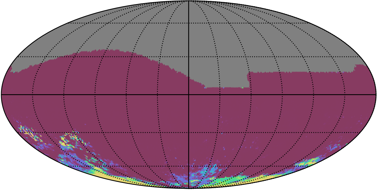
roll_pause_mjdp365_v3.4_10yrs All sky ri bands: 75th Percentile Intranight Timespan
