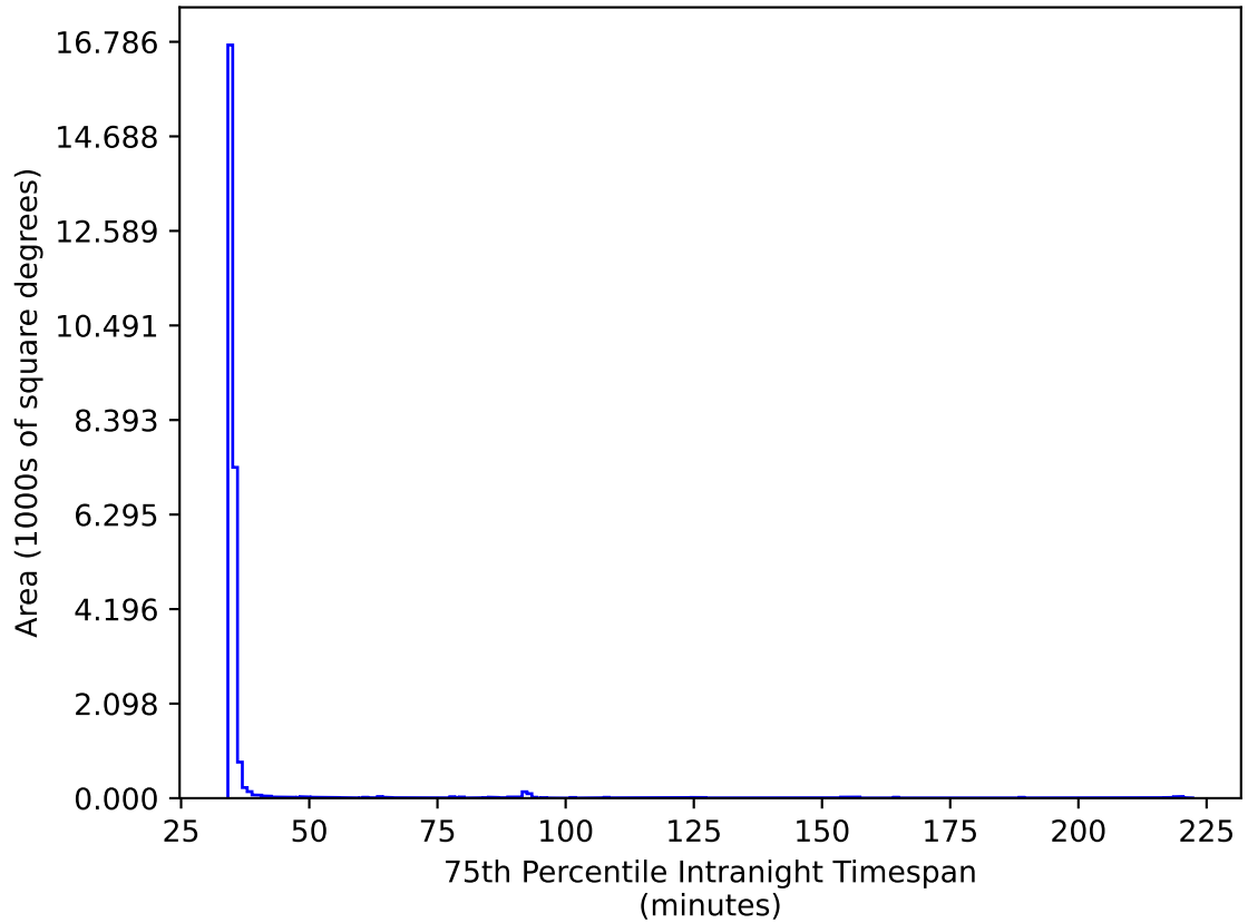
roll_pause_mjdp365_v3.4_10yrs All sky ri bands: 75th Percentile Intranight Timespan
