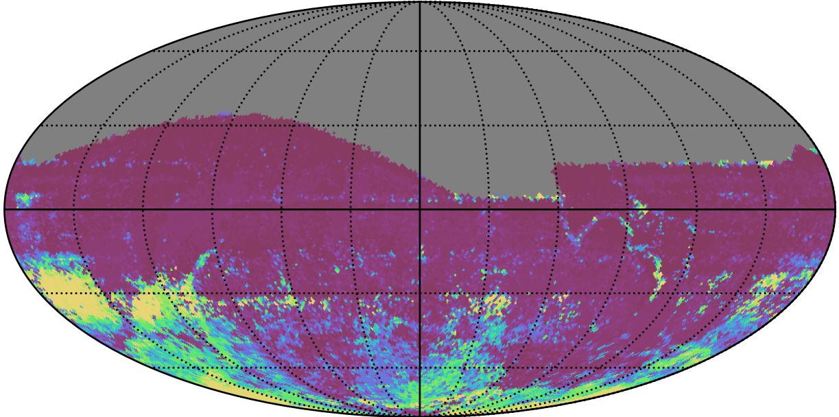
roll_pause_mjdp365_v3.4_10yrs All sky r band: 75th Percentile Intranight Timespan
