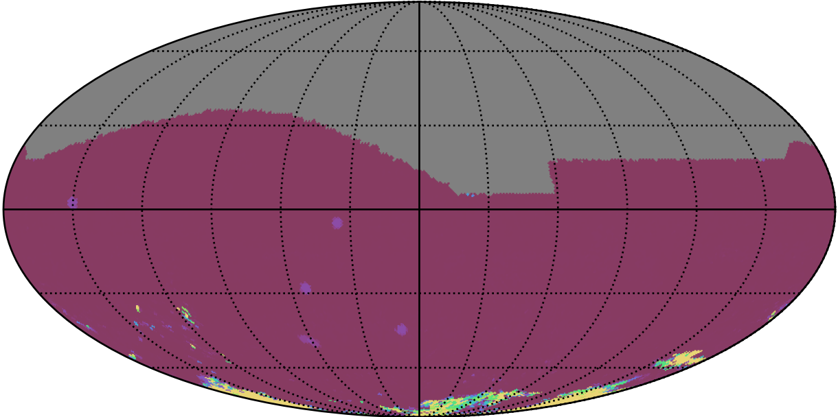
roll_pause_mjdp365_v3.4_10yrs All sky iz bands: 75th Percentile Intranight Timespan
