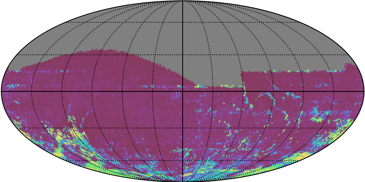
roll_pause_mjdp365_v3.4_10yrs All sky i band: 75th Percentile Intranight Timespan
