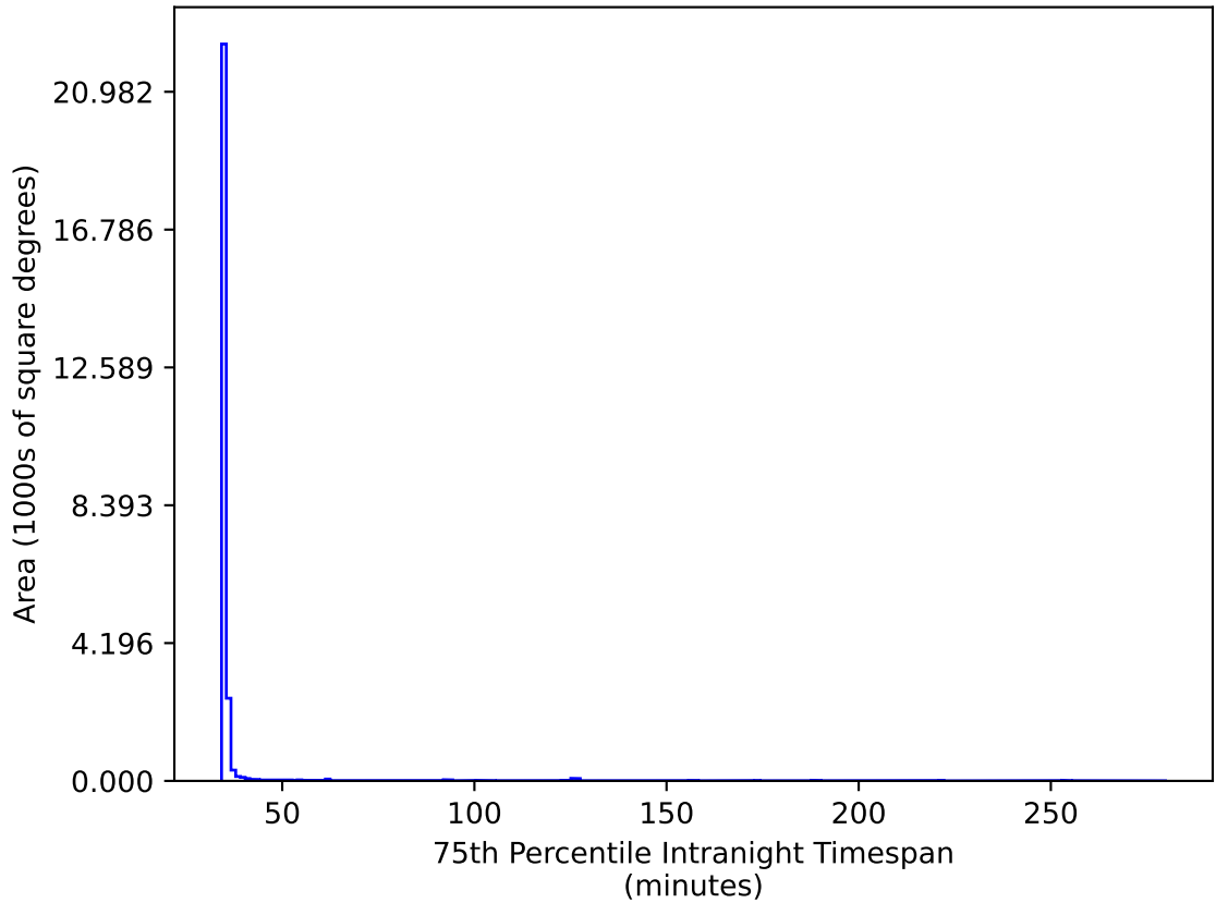
roll_pause_mjdp365_v3.4_10yrs All sky gr bands: 75th Percentile Intranight Timespan
