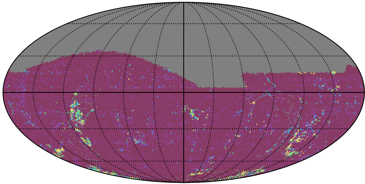
roll_pause_mjdp365_v3.4_10yrs All sky g band: 75th Percentile Intranight Timespan
