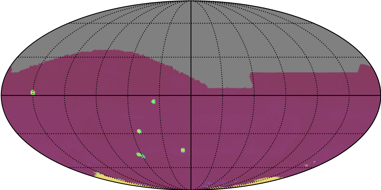
roll_pause_mjdp365_v3.4_10yrs All sky all bands: 75th Percentile Intranight Timespan
