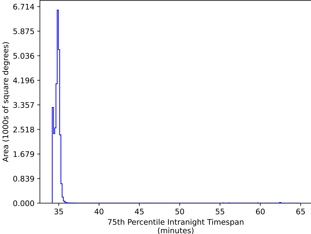
roll_pause_mjdp365_v3.4_10yrs All sky all bands: 75th Percentile Intranight Timespan
