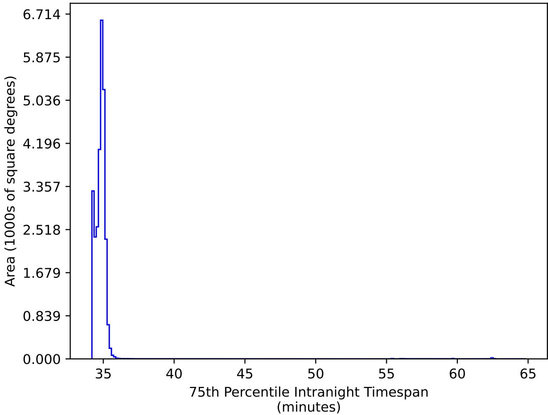
roll_pause_mjdp365_v3.4_10yrs All sky: 75th Percentile Intranight Timespan
