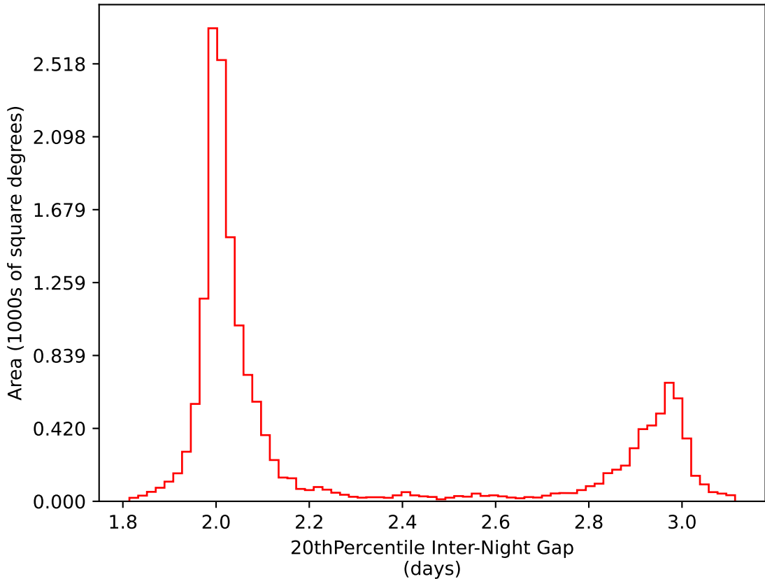
roll_pause_mjdp365_v3.4_10yrs WFD i band: 20thPercentile Inter-Night Gap
