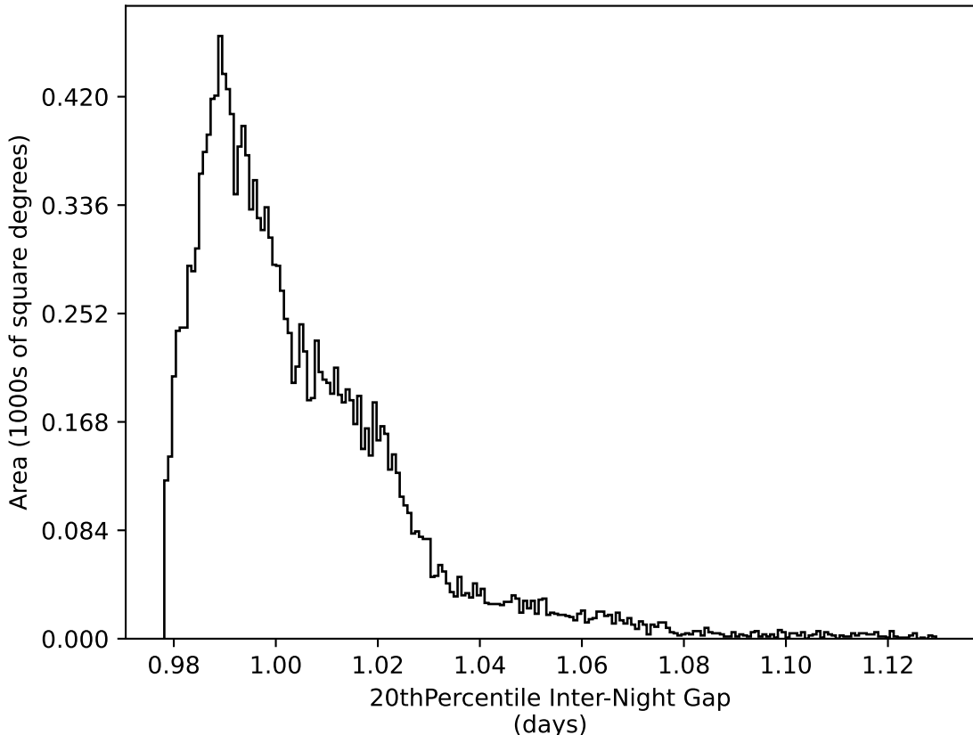
roll_pause_mjdp365_v3.4_10yrs WFD all bands: 20thPercentile Inter-Night Gap
