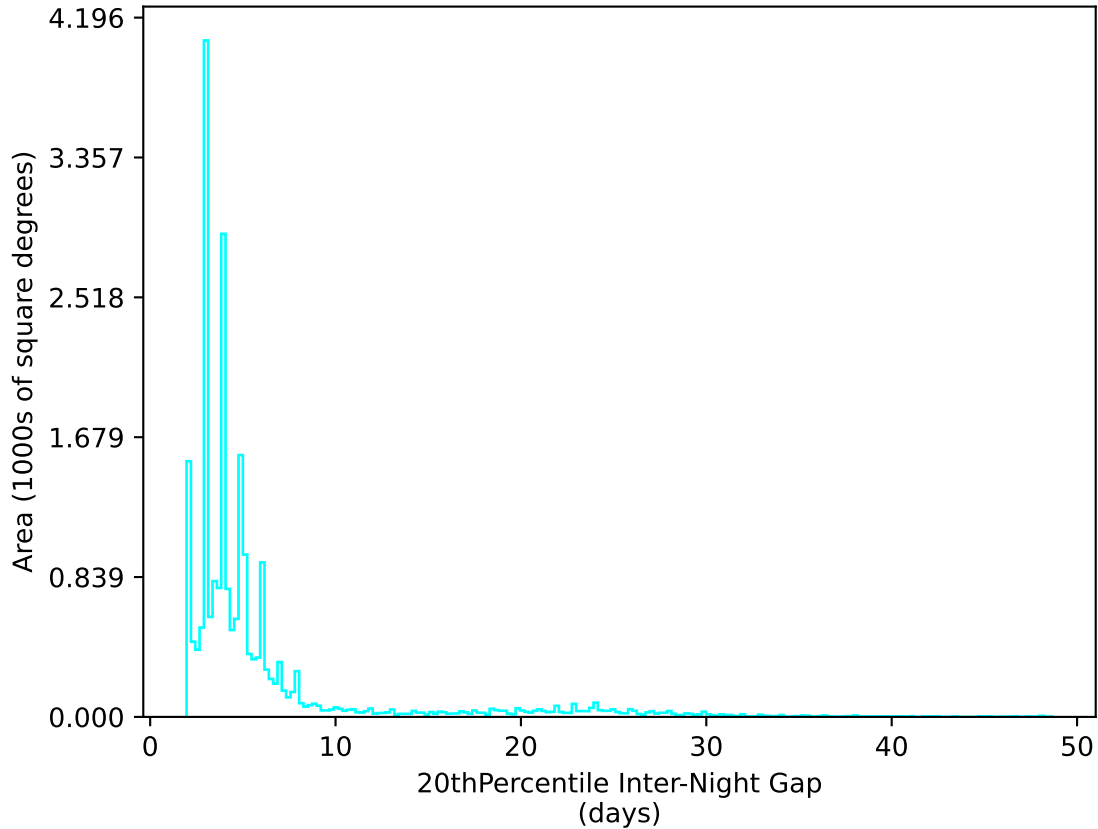
roll_pause_mjdp365_v3.4_10yrs All sky u band: 20thPercentile Inter-Night Gap
