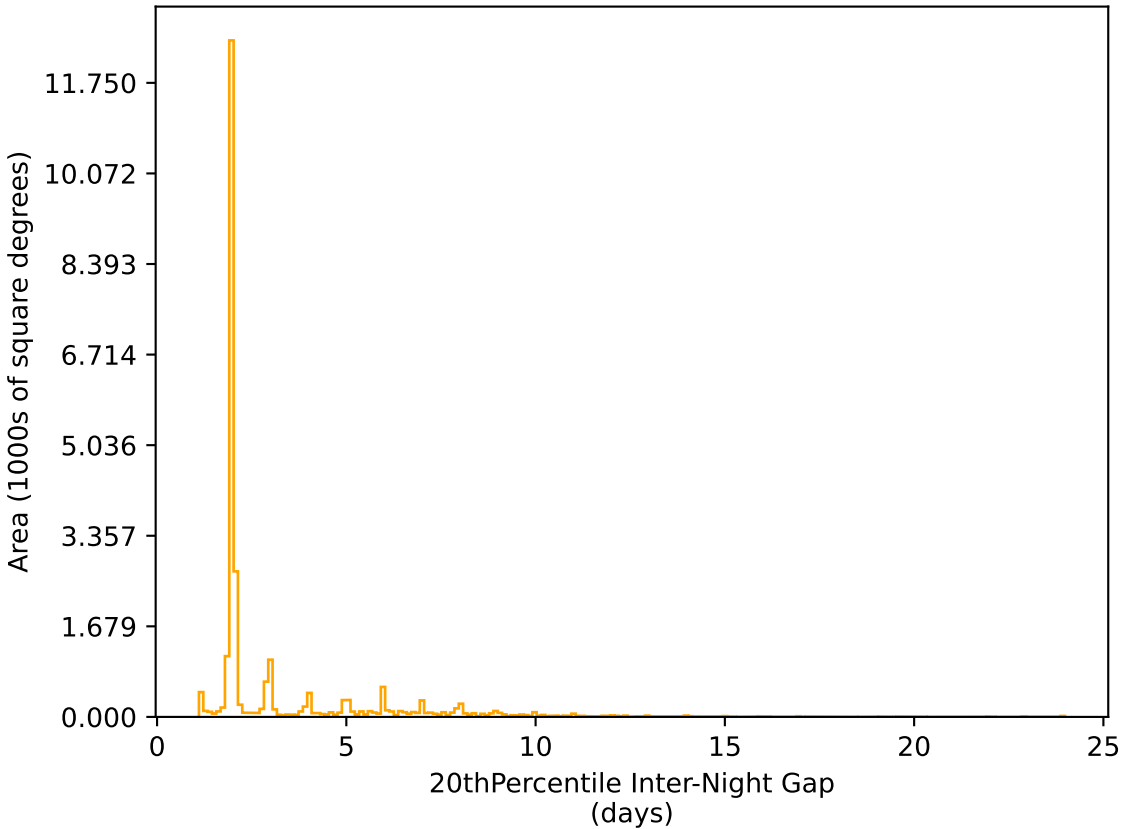
roll_pause_mjdp365_v3.4_10yrs All sky r band: 20thPercentile Inter-Night Gap
