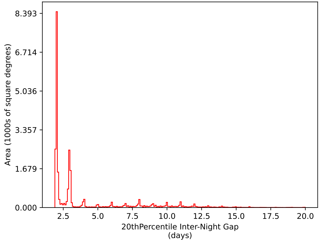
roll_pause_mjdp365_v3.4_10yrs All sky i band: 20thPercentile Inter-Night Gap
