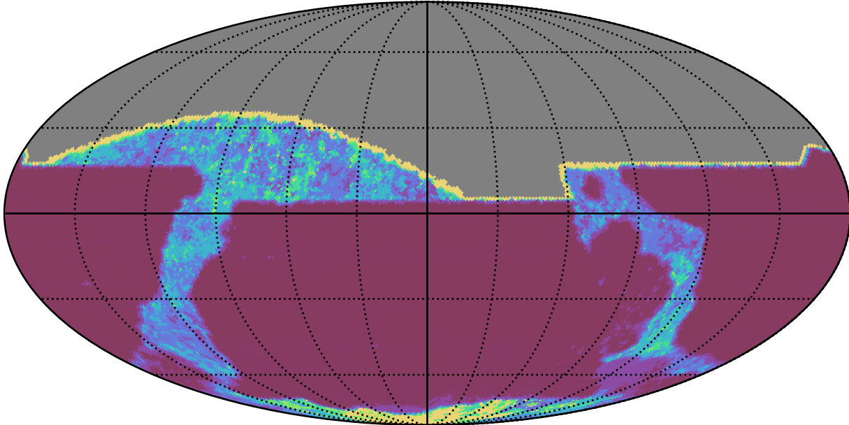
roll_pause_mjdp365_v3.4_10yrs All sky all bands: 20thPercentile Inter-Night Gap
