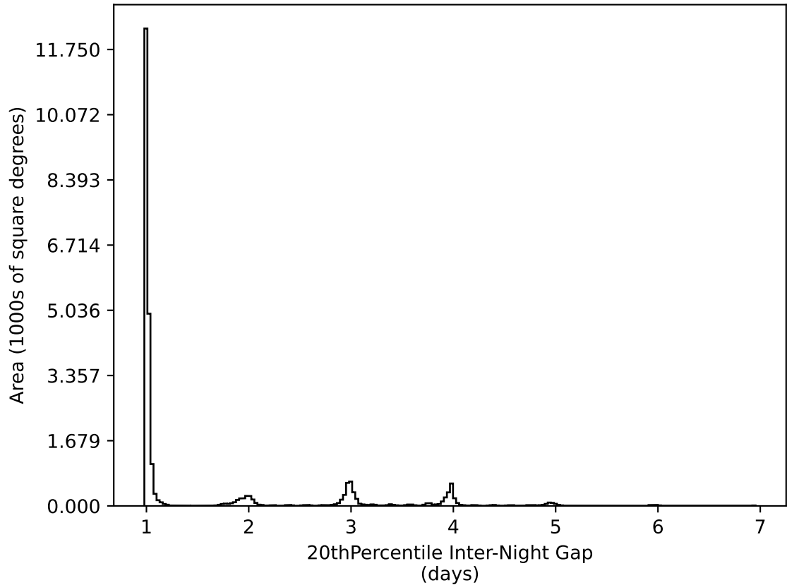
roll_pause_mjdp365_v3.4_10yrs All sky all bands: 20thPercentile Inter-Night Gap
