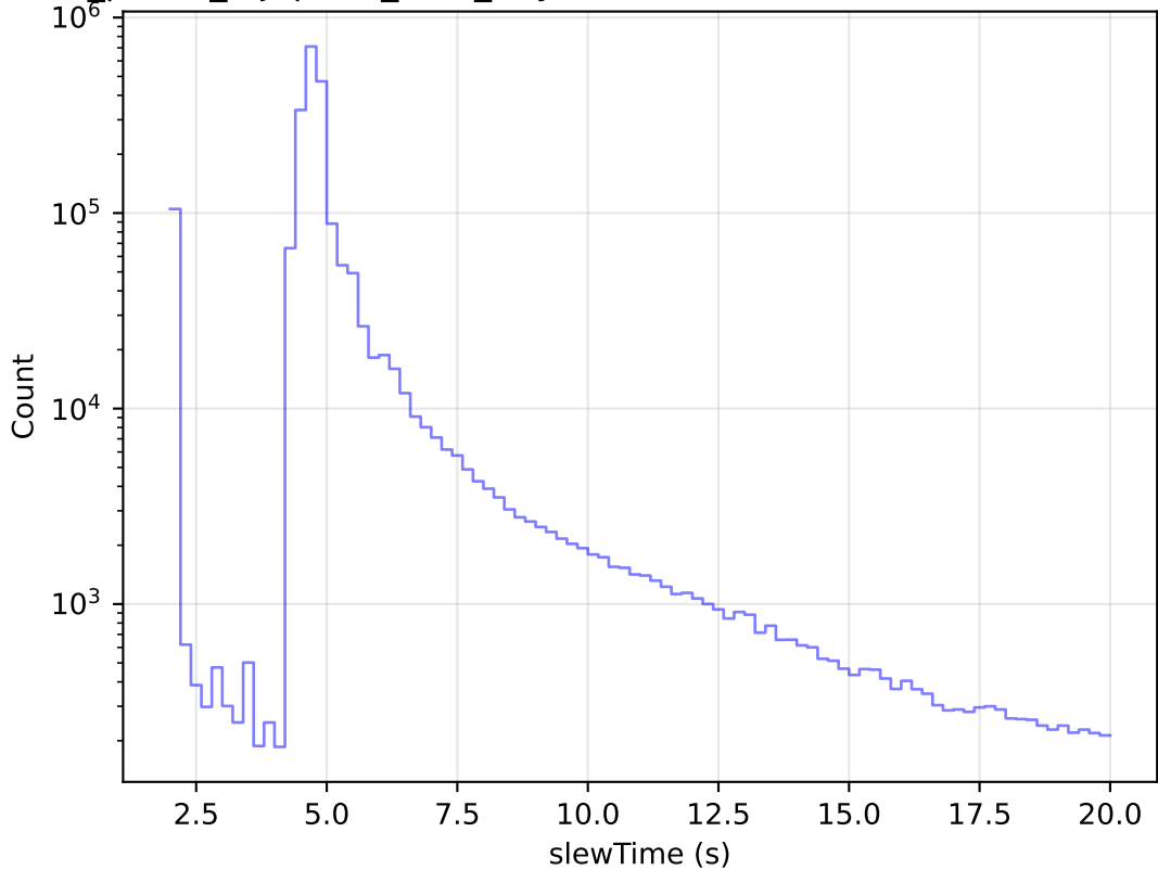
roll_pause_mjdp365_v3.4_10yrs All visits: Zoom Slew Time Histogram
