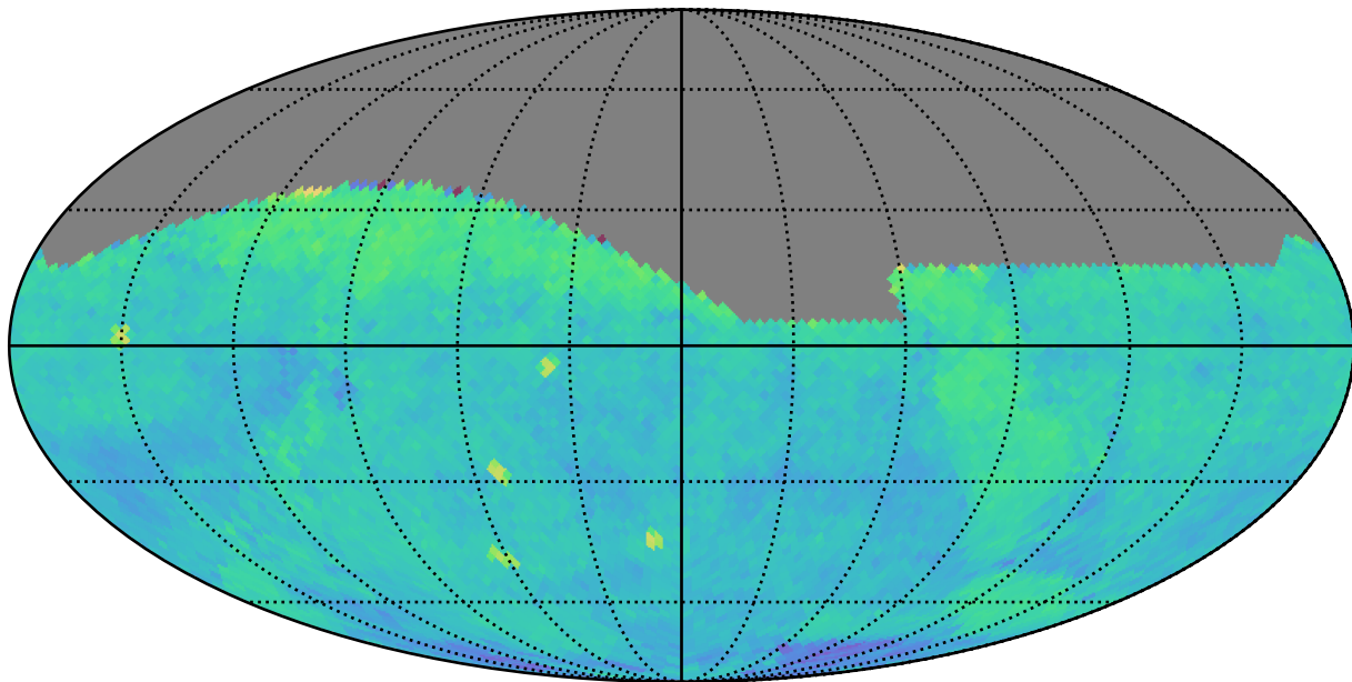
roll_pause_mjdp365_v3.4_10yrs (g or r or i): PairFraction
