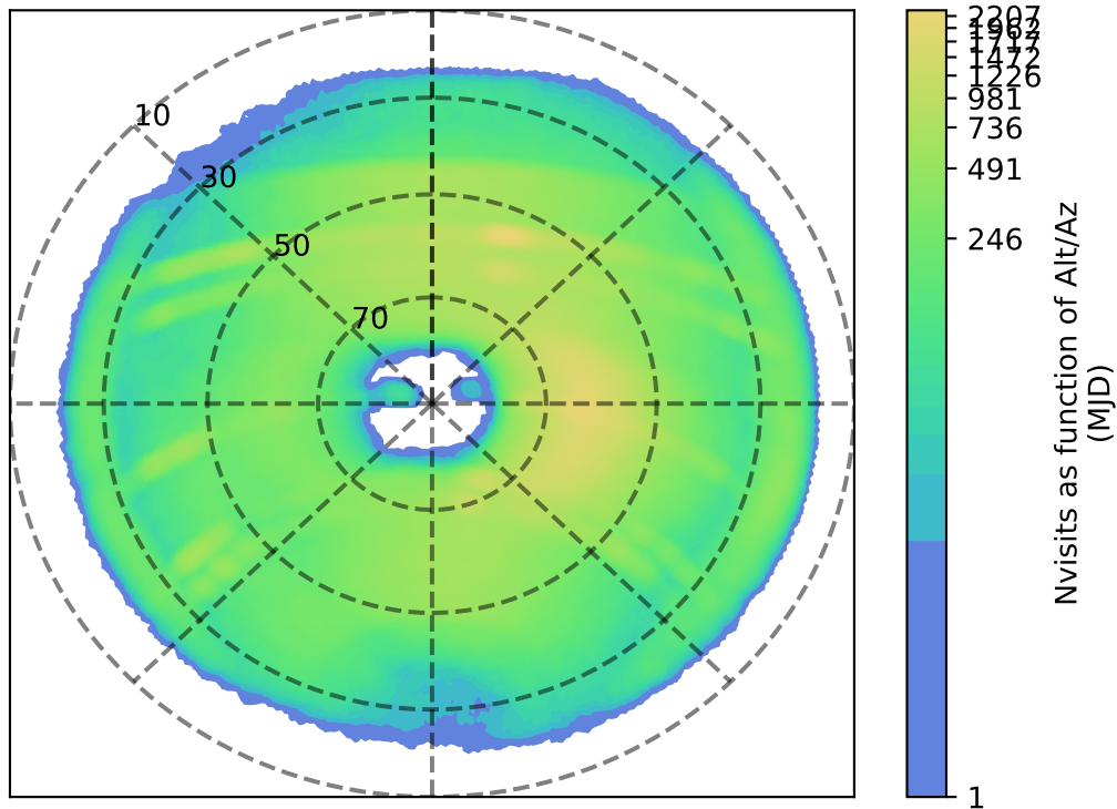
roll_pause_mjdp365_v3.4_10yrs z: Nvisits as function of Alt/Az
